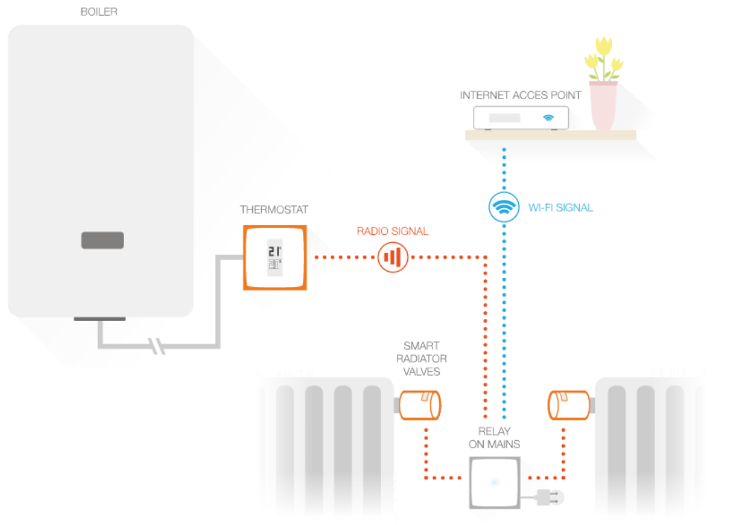
Smart Valves paired with the Relay of the Smart Thermostat
