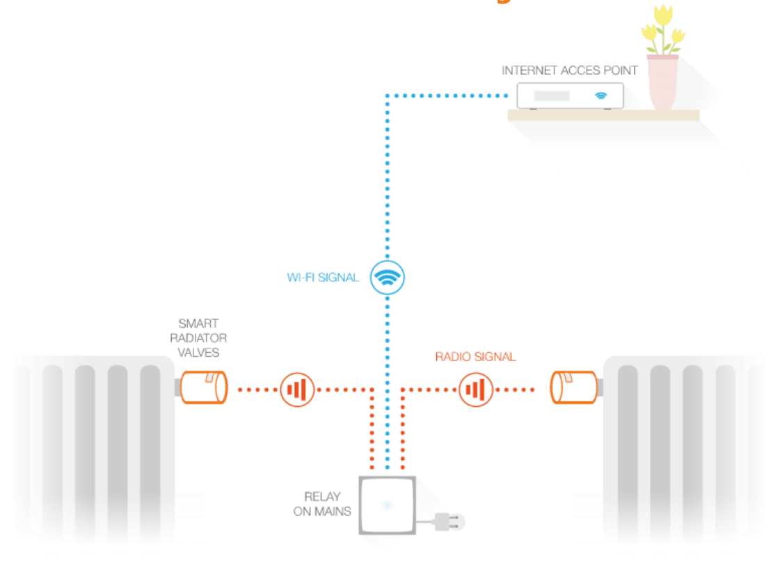
Smart Valves paired with the Relay of the Starter Pack
